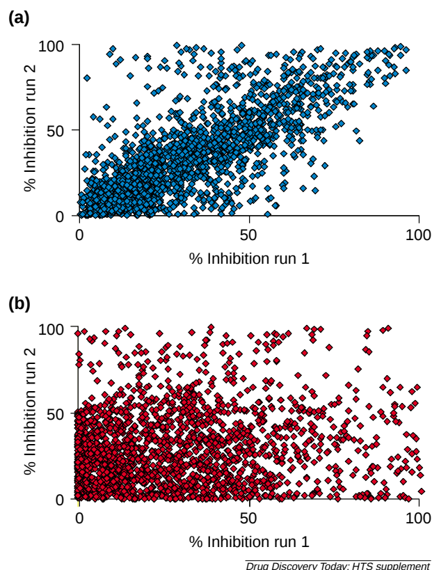
Figure 6. Two hypothetical HTS assays undertaken in duplicate illustrating potential SAR patterns (or the lack of them). (a) depicts an assay with high reproducibility and (b) depicts an assay with low reproducibility.
